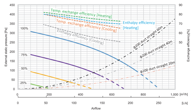
DIAGRAM LGH-65RVX3-E
