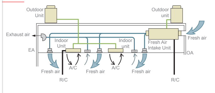
OPERATING SCHEME - EXAMPLE
