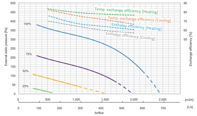
DIAGRAM LGH-200RVX3-E
